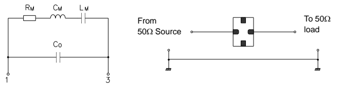
Equivalent LC Model
